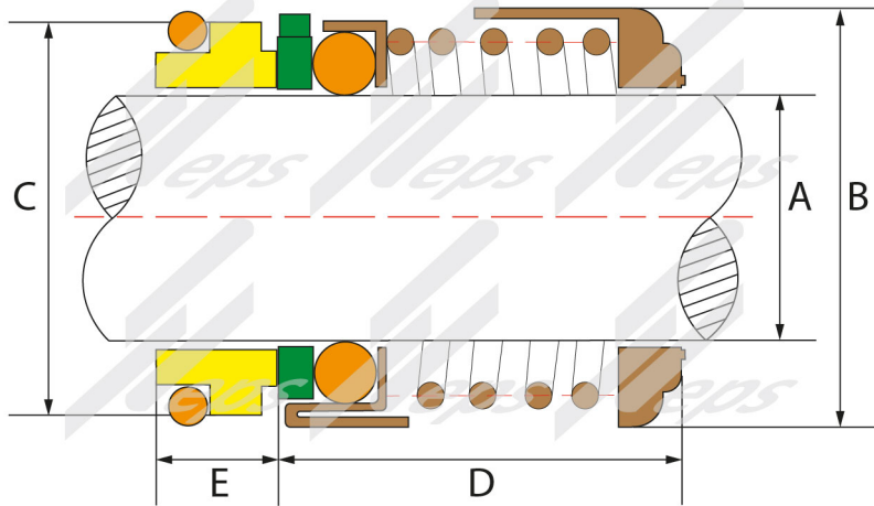
EPSGR-CHI 12 mm
