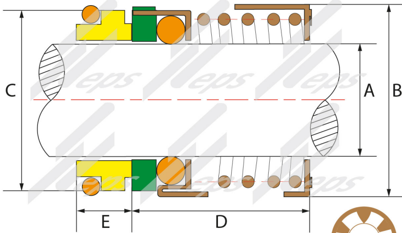
EPSGR-CHI 16 mm
